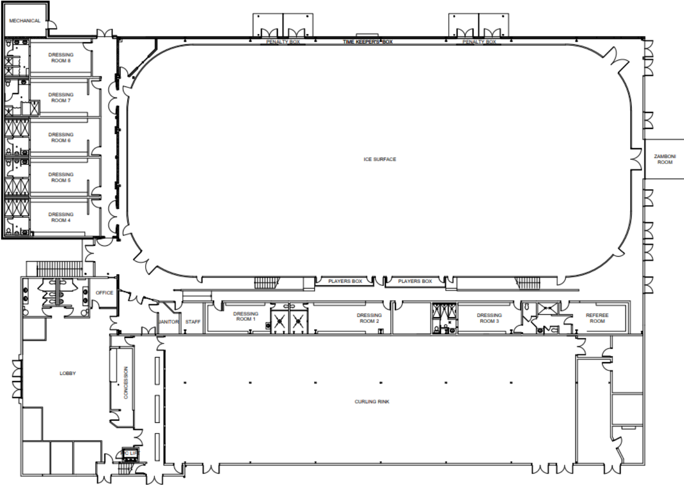
ICE SURFACE FLOOR PLAN
